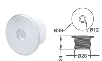
φ1-1/2" Face (Standard) Jet
